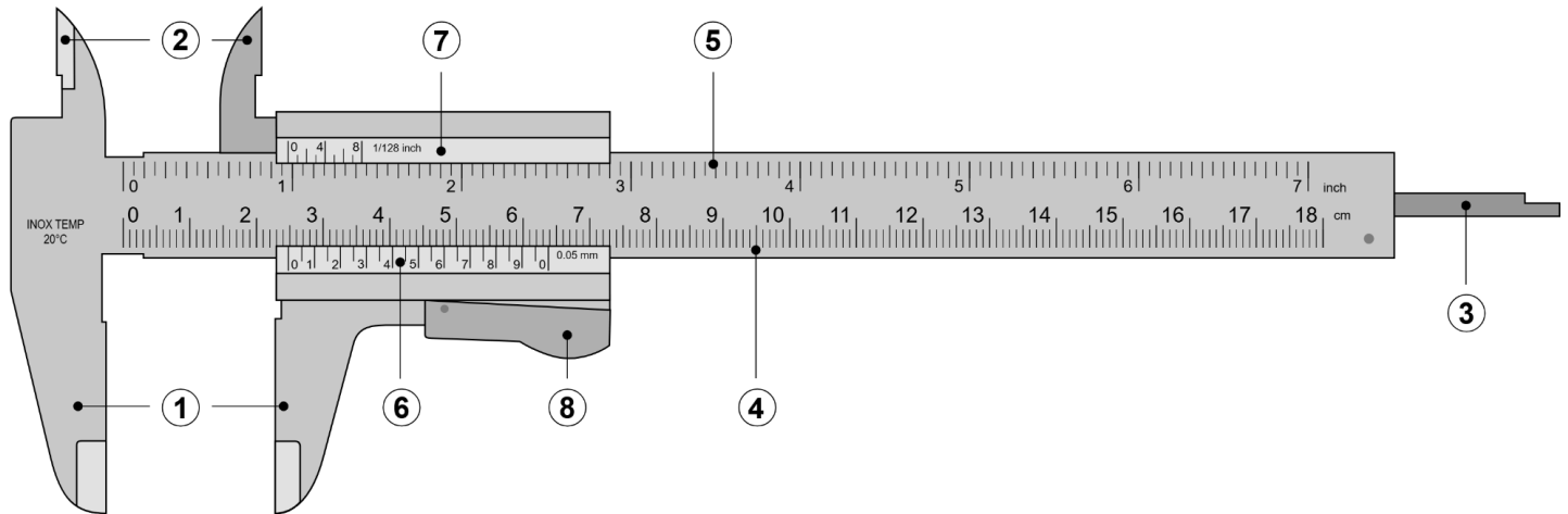
Figure 1.2. Parts of a Vernier Caliper.
